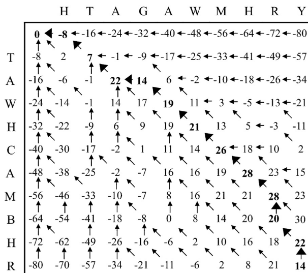
Figure 7. The global dynamic programming matrix for hypercomplex number representation of DNA sequences.
